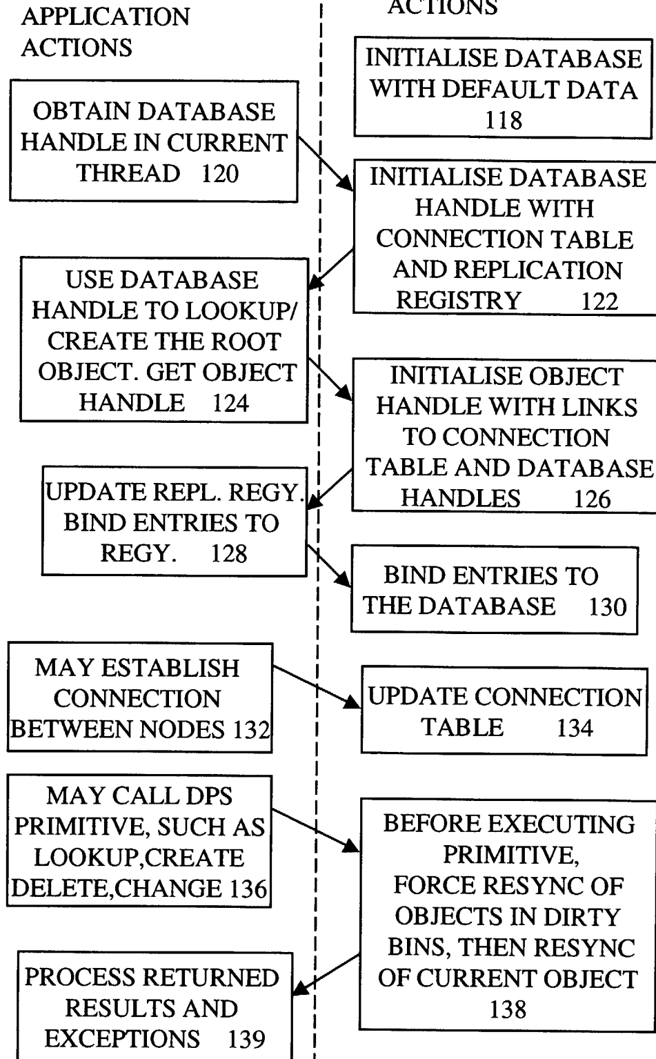
FIG 8 DPS MIDDLEWARE ACTIONS
