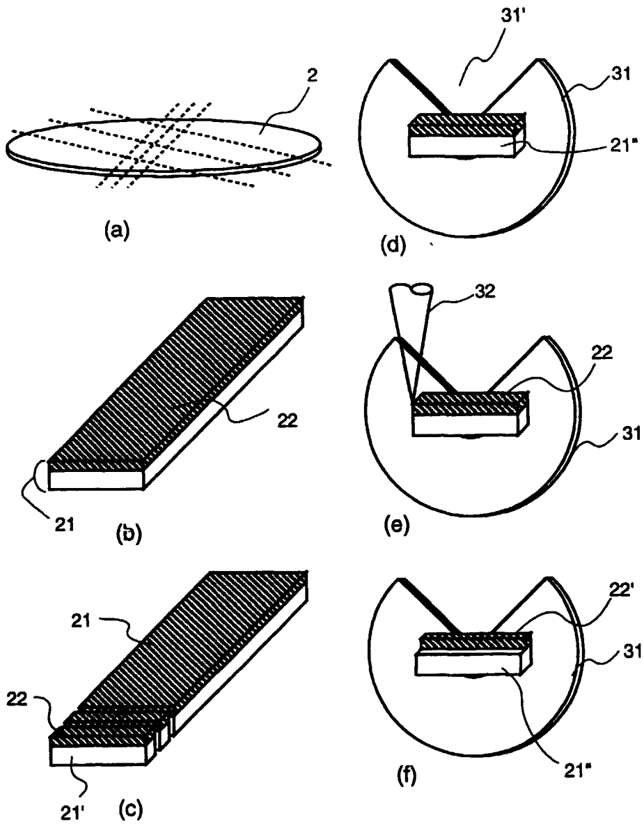
FIG.3 (PRIOR ART)
