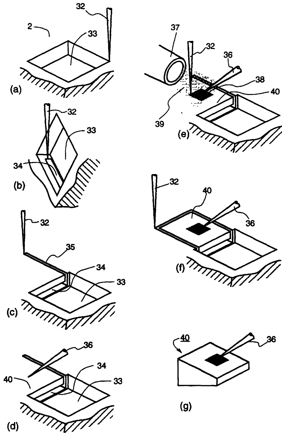
FIG.4 (PRIOR ART)
