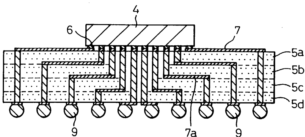
Fig.28 PRIOR ART
