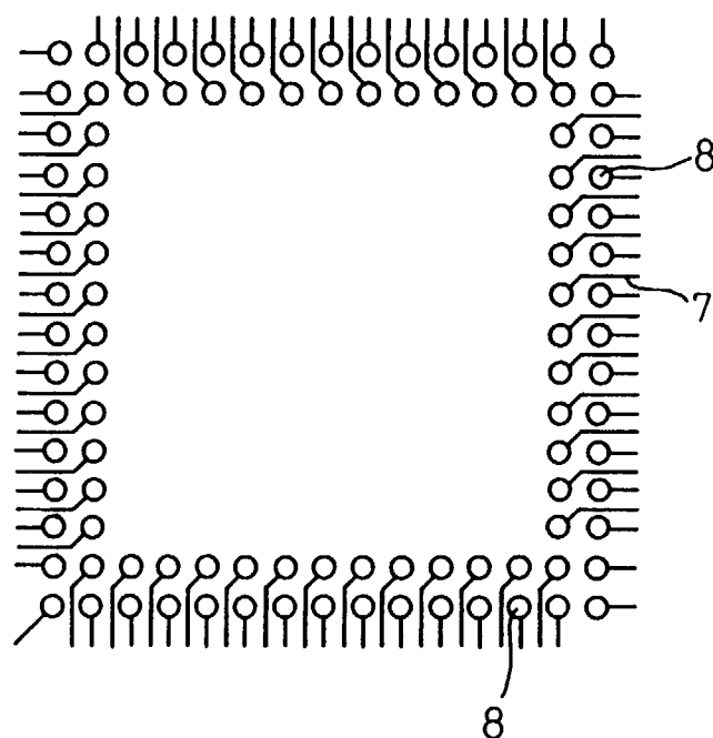
Fig.27 PRIOR ART
