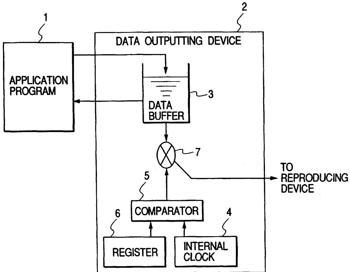
FIG. 1 PRIOR ART
