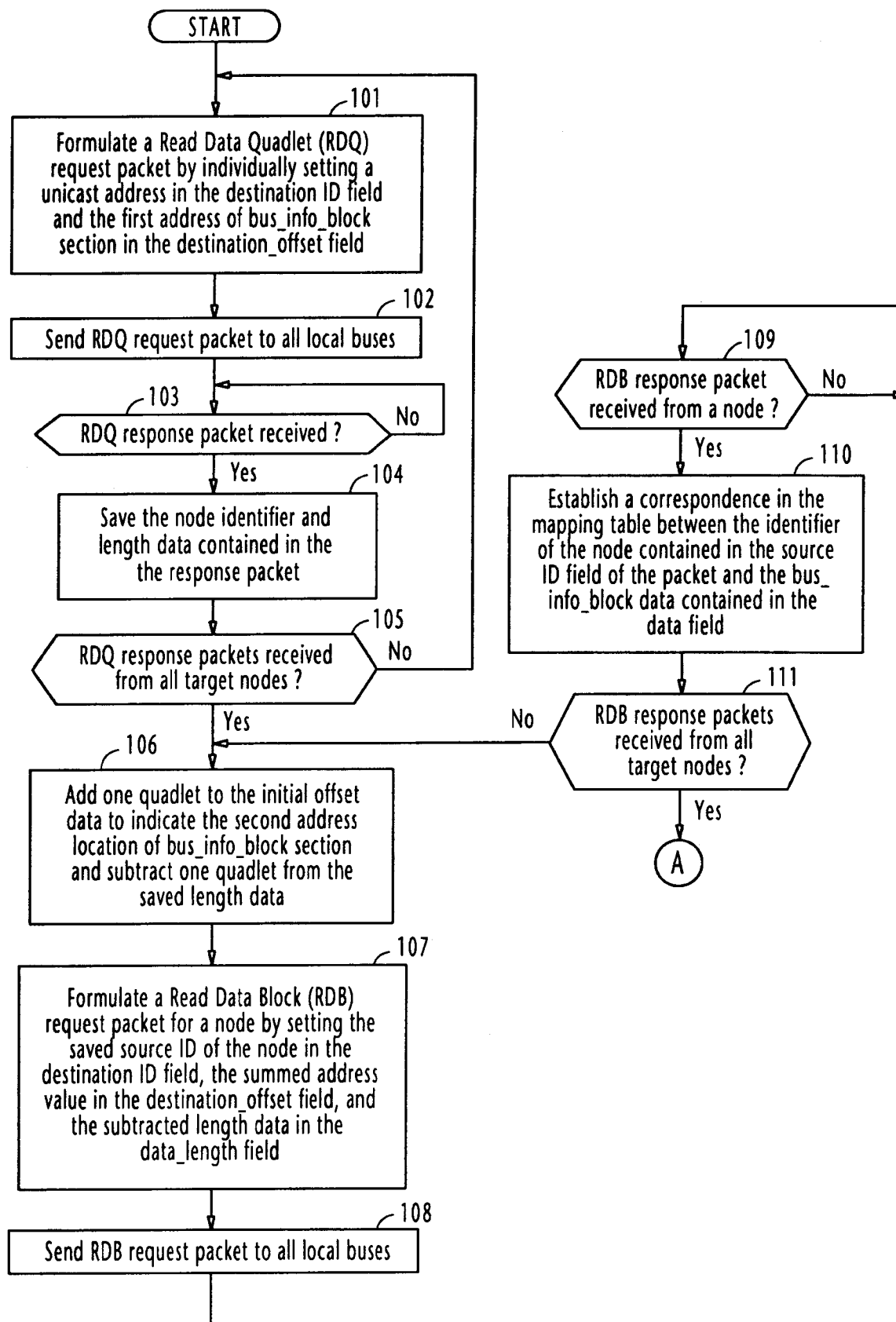
FIG. 4A BUS_INFO_BLOCKS
