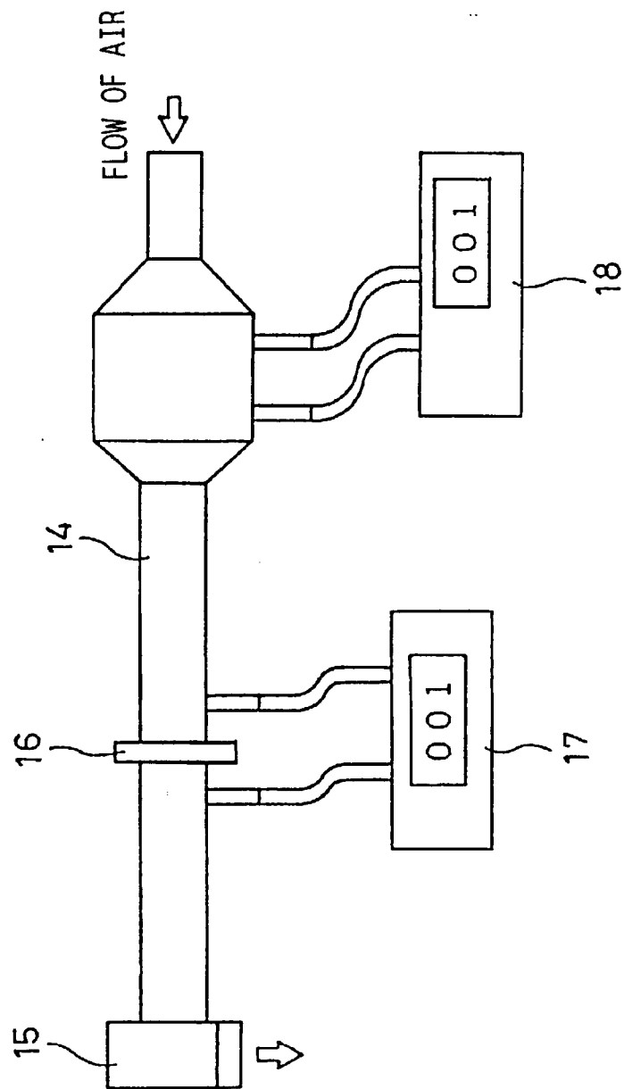
FIG. 3 MEASURING DEVICE
