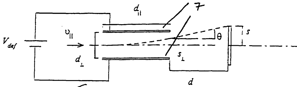
Figure 3: A model of electrostatic deflectors
