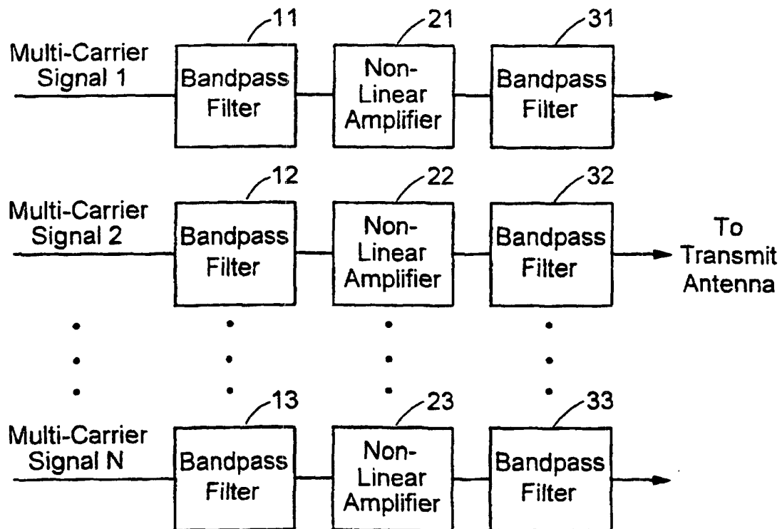
FIG. 6 (Prior Art)
