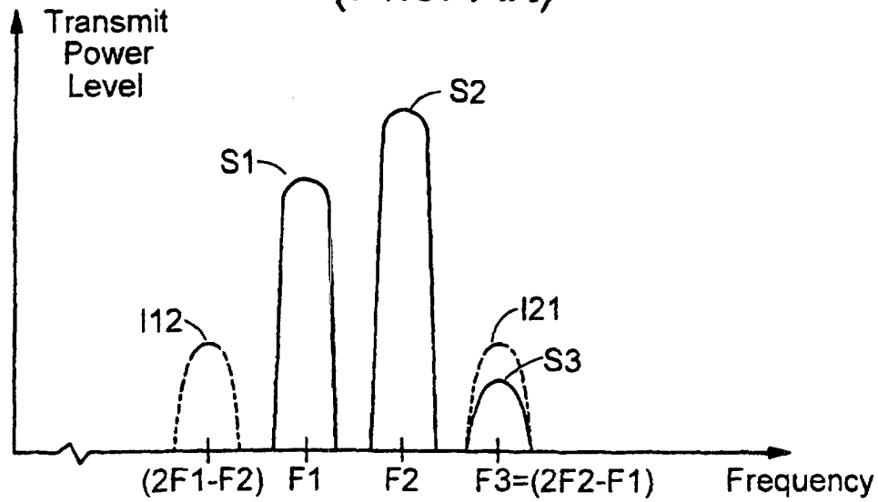
FIG. 5 (Prior Art)
