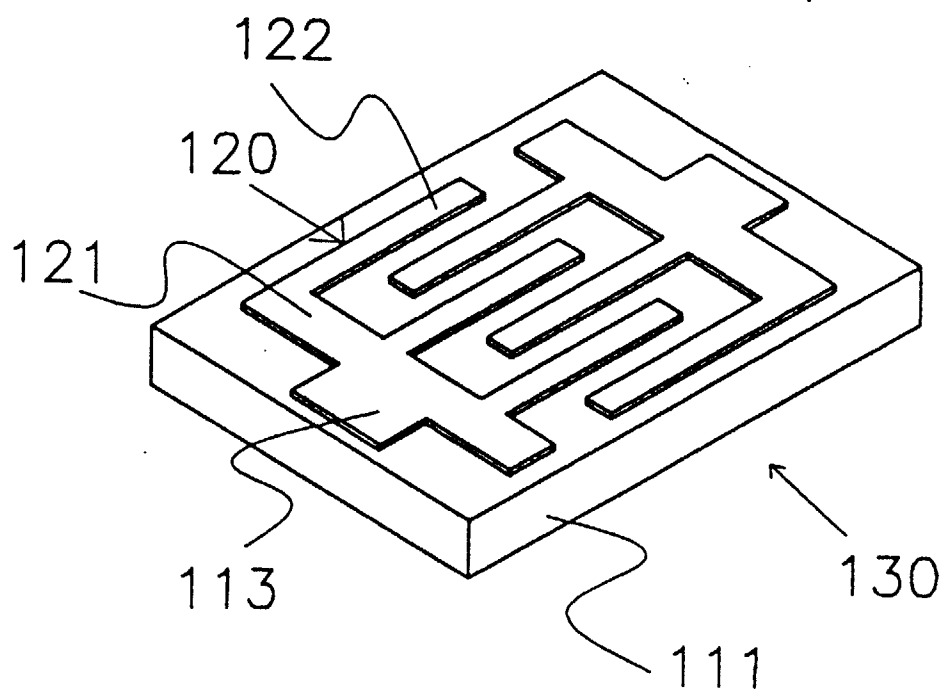
FIG. 6 PRIOR ART
