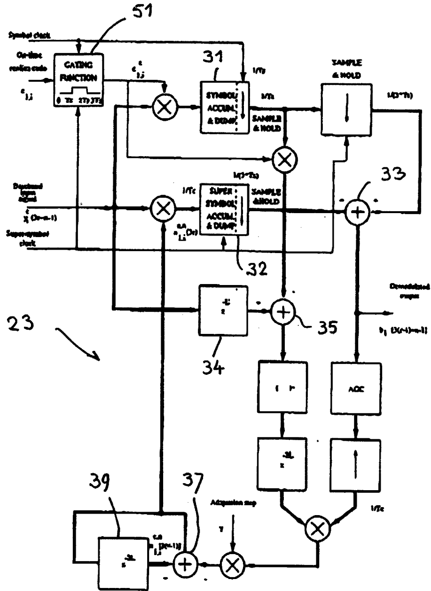
Baseline EC-BAID-II detector functional block diagram
