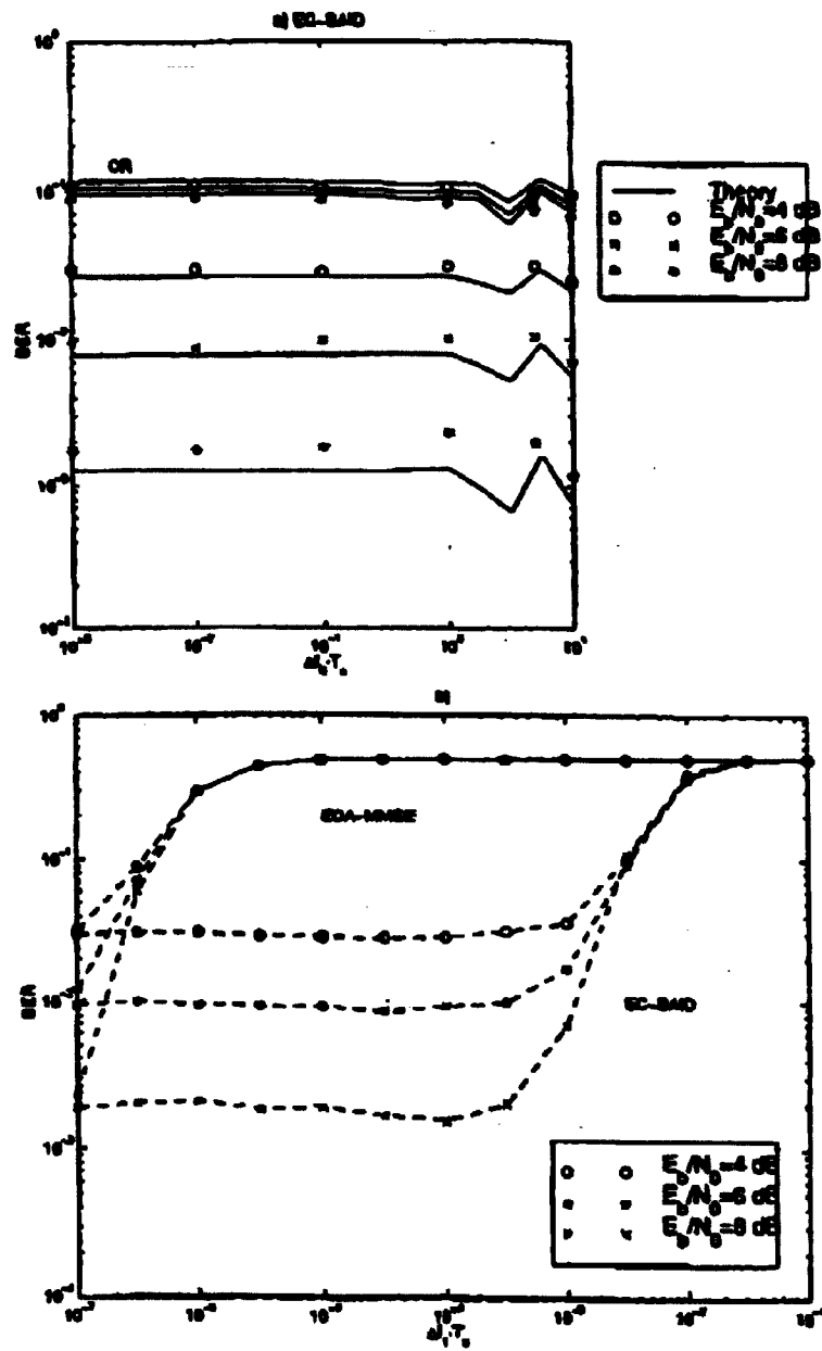
a) BER vs. \Delta f_1 \cdot T , for EC-BAID detector: L = 64 , K = 19 , [C/I]_{sc} = -6 dB, b) BER vs. \Delta f_1 \cdot T , for different detectors: BPSK-RS, L = 64 , K = 19 , [C/I]_{sc} = -6 dB
