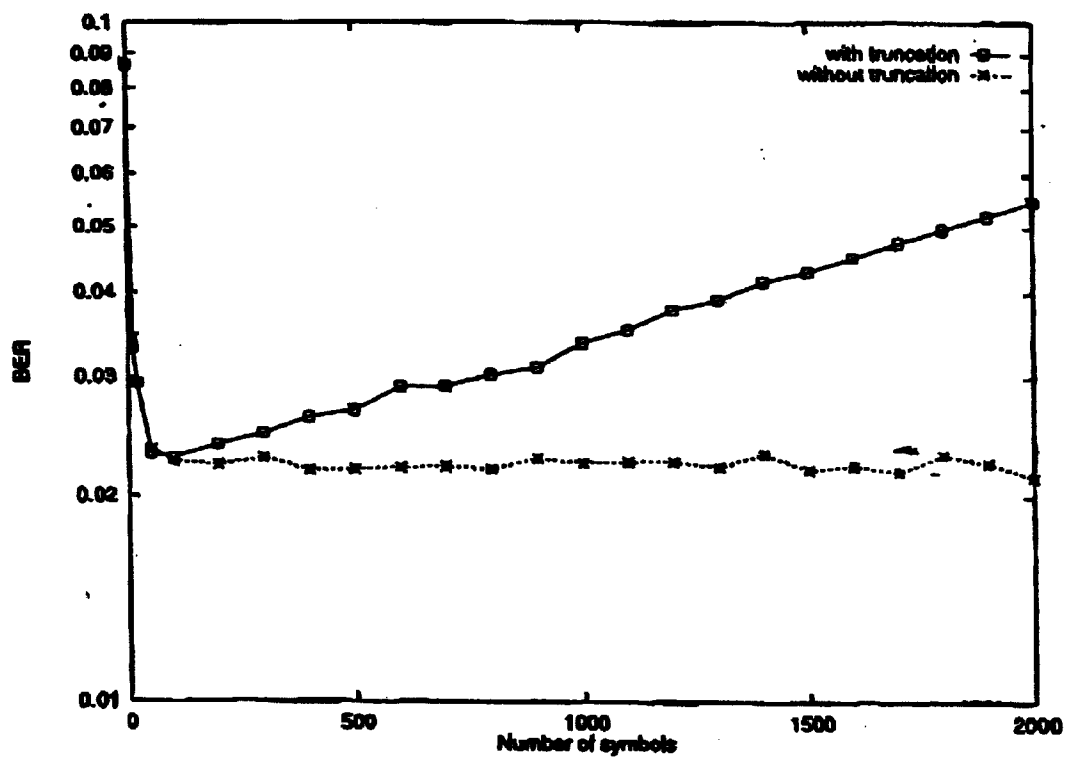
BER system performance with and without error signal truncation effects for L = 128 , N = 64 , E_s/N_0 = 6 dB and C/I = -6 db.
