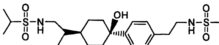
Example 37; Cis
