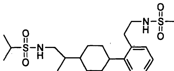
ortho-substituted
