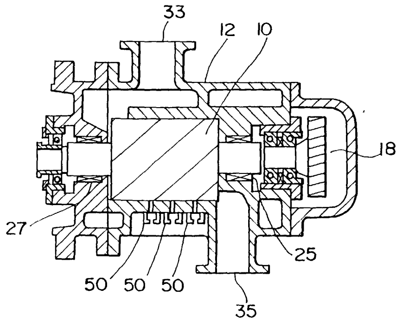
Fig.4 PRIOR ART
