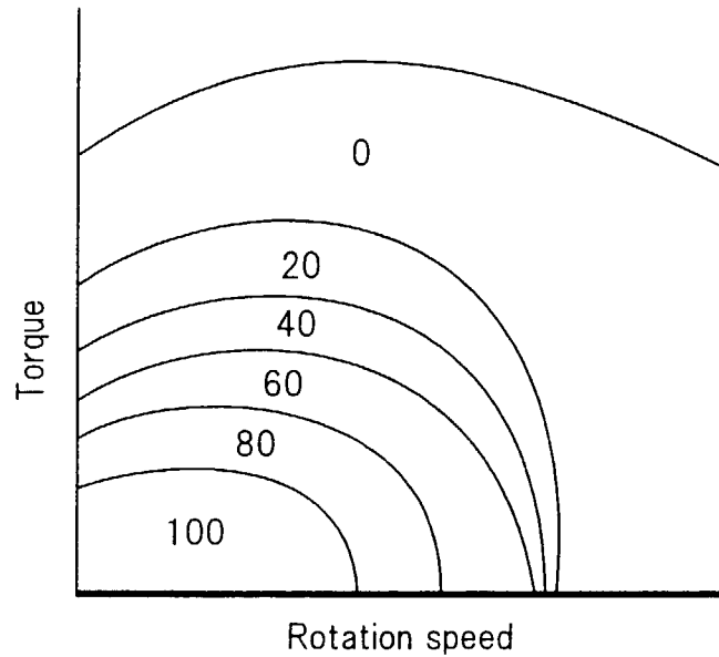
Target EGR Map
