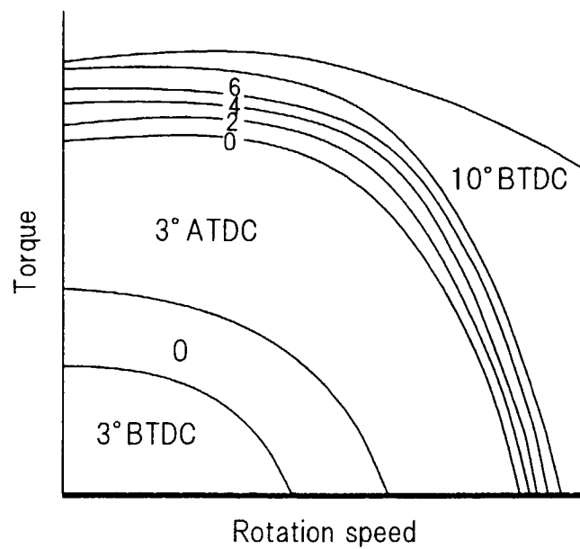
Main injection timing Map
