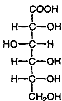
D-gluconic acid
