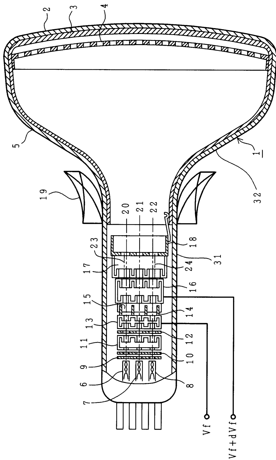
FIG. 11 (PRIOR ART)
