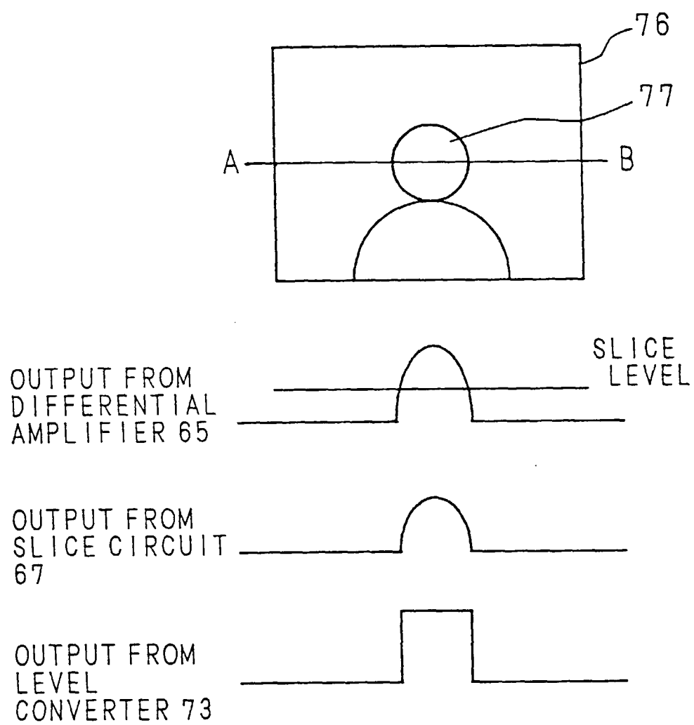
Fig. 7 Prior Art
