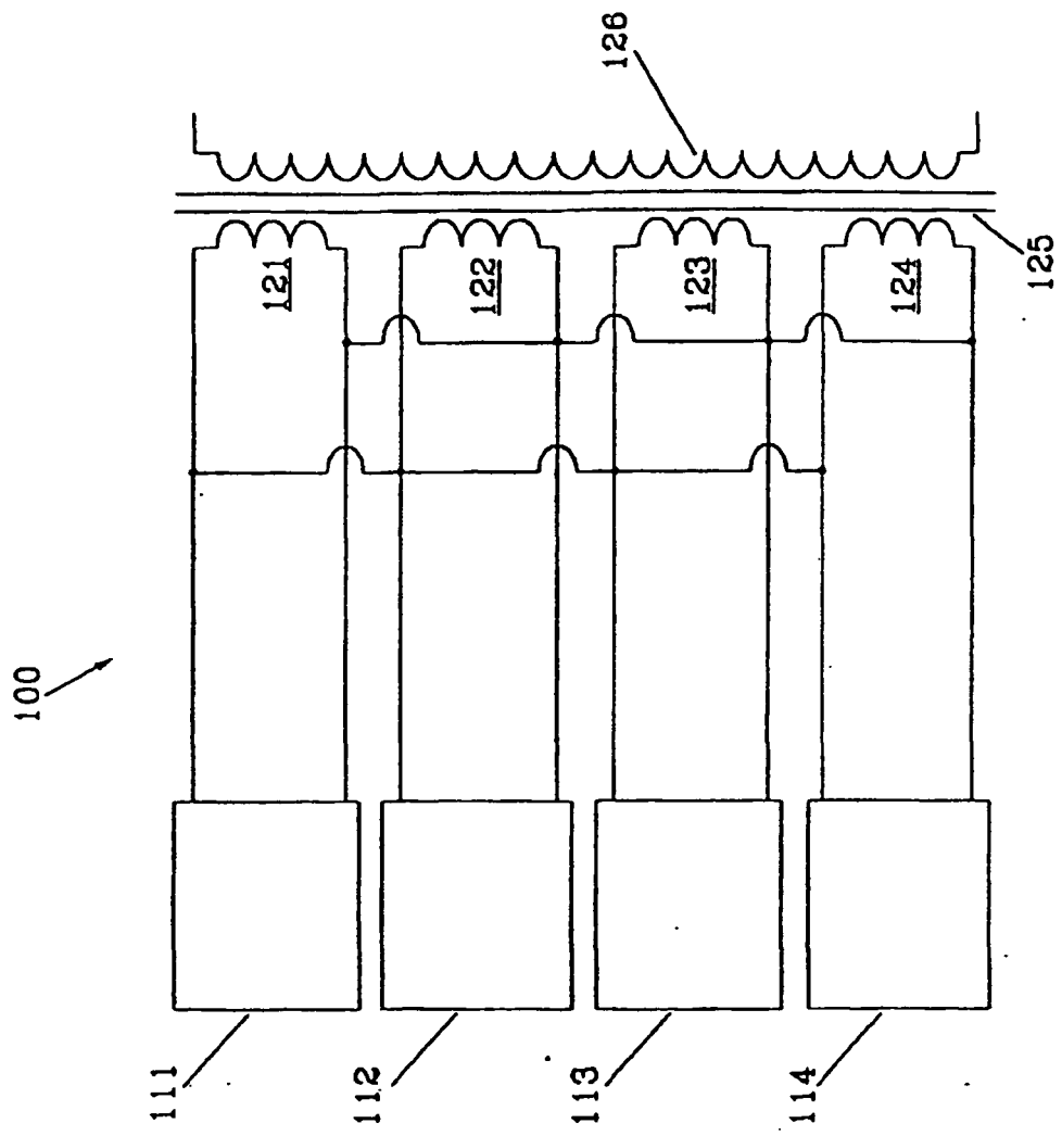
Fig. 11 (Prior art)
