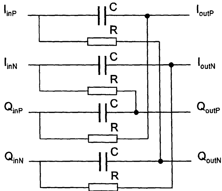
Fig. 5 (prior art)
