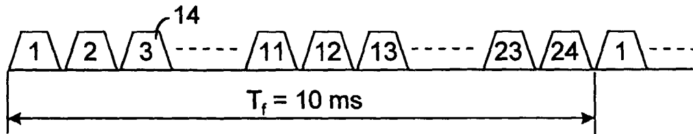
Fig. 2 (prior art)
