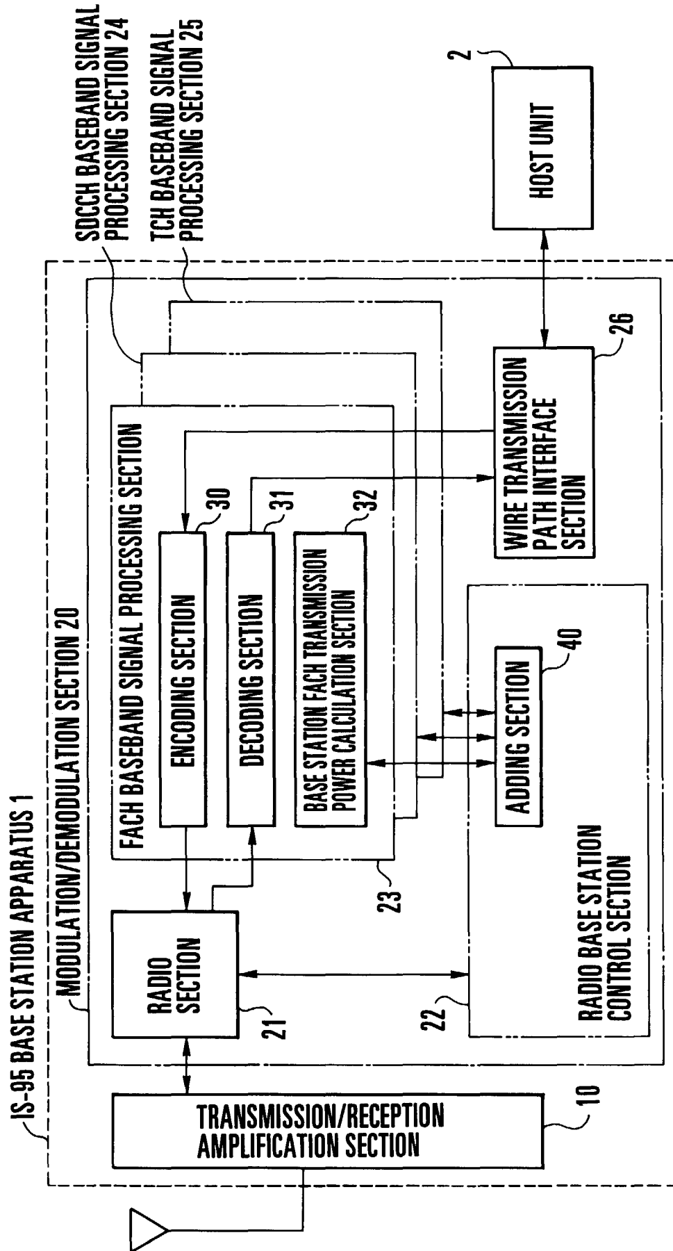
FIG. 20 PRIOR ART
