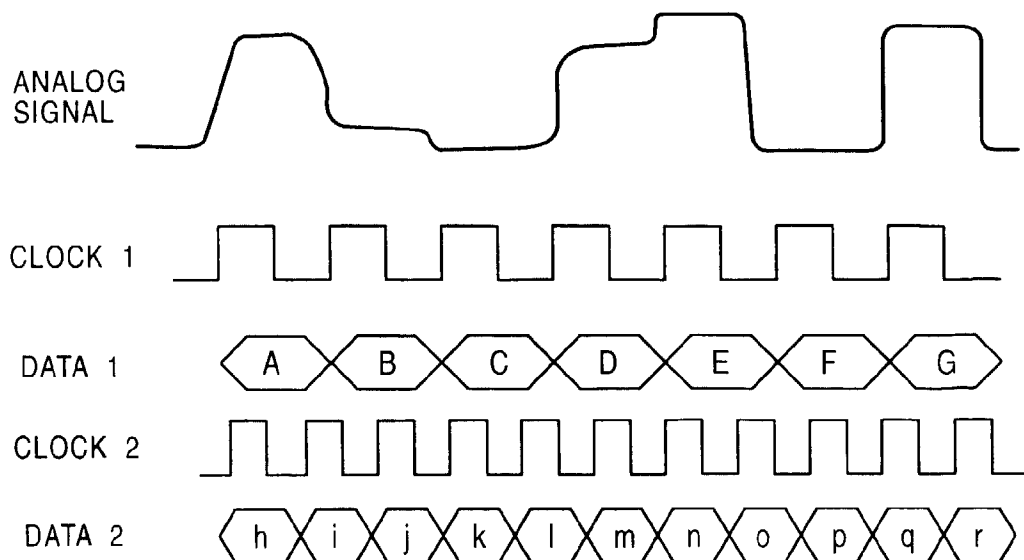
FIG. 9 PRIOR ART
