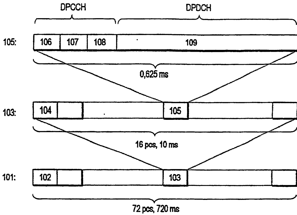
Fig. 1 PRIOR ART
