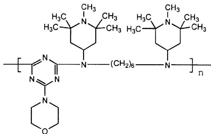
Structural Formula I
