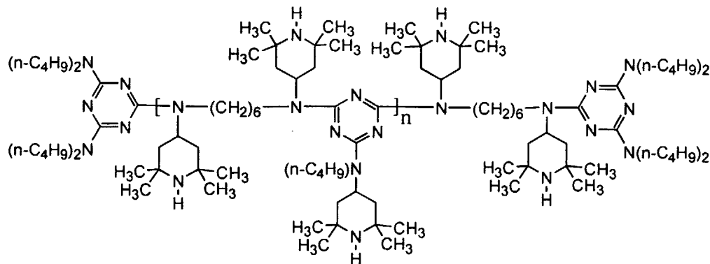
Structural Formula II
