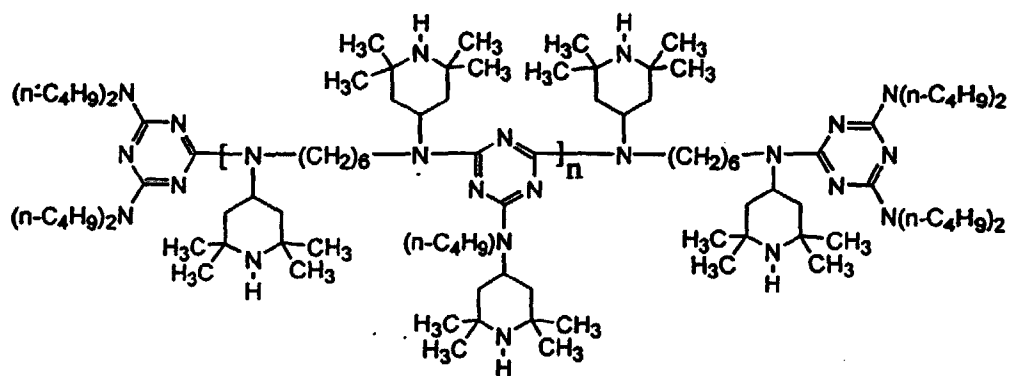
Structural Formula II
