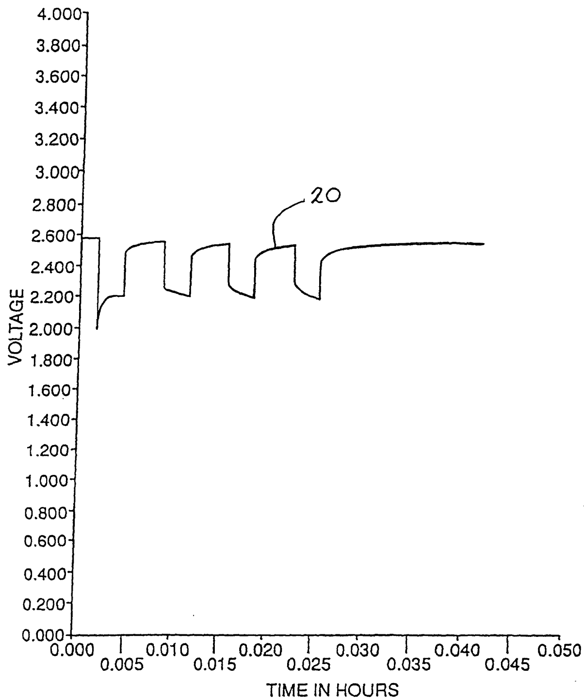
FIG. 3 (PRIOR ART)
