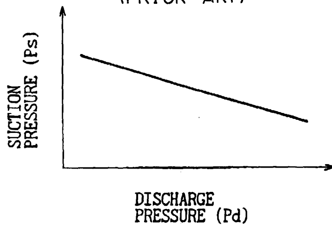
Fig.15 (PRIOR ART)
