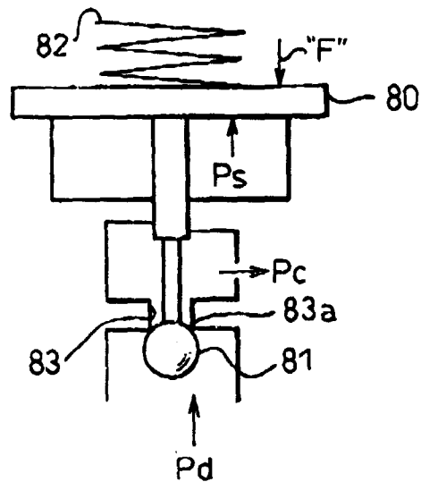
Fig.14 (PRIOR ART)
