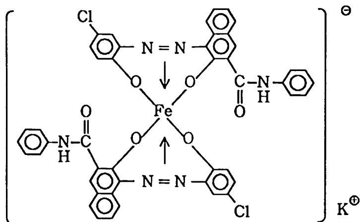
Formula (a)
