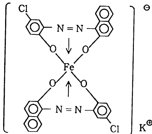
Formula (b)
