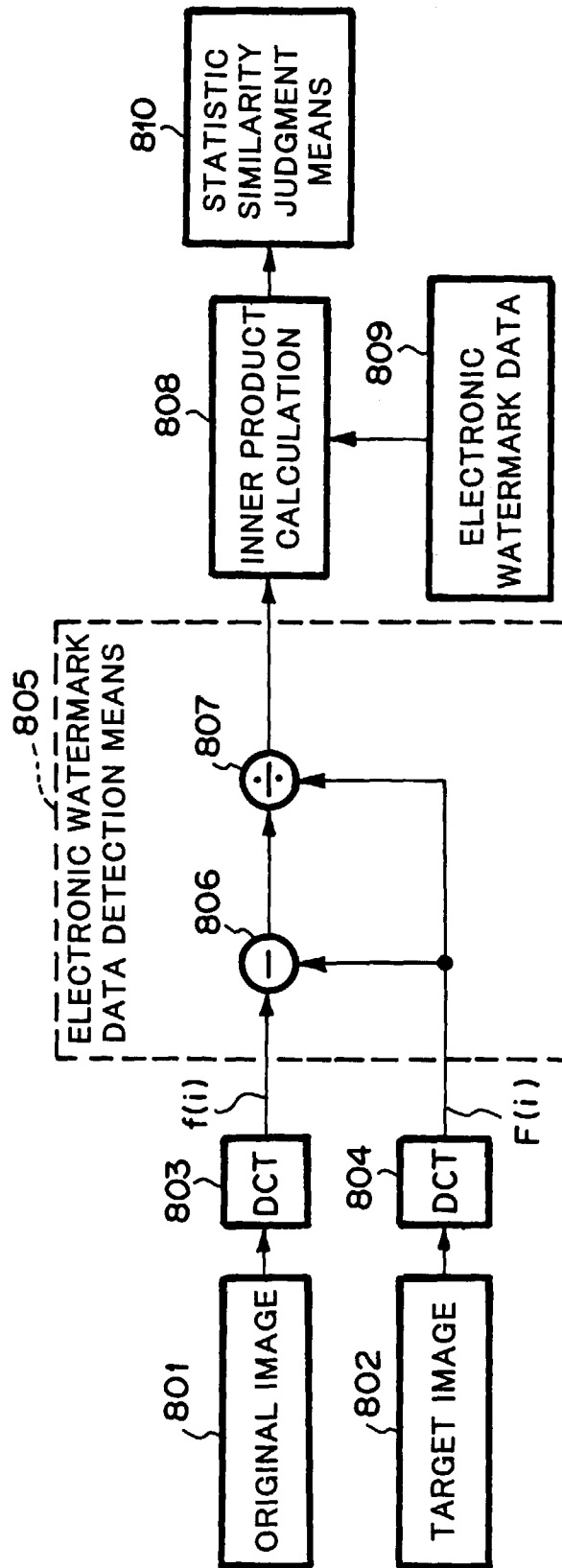
FIG. 8 (PRIOR ART)
