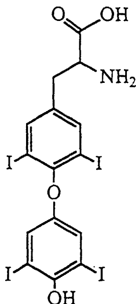
FORMULA 1 L- AND D- THYROXINE
