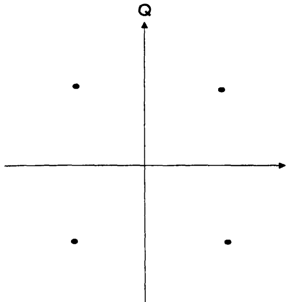
COMBINED SIGNAL CONSTELLATION WITH NO INTERFERENCE
