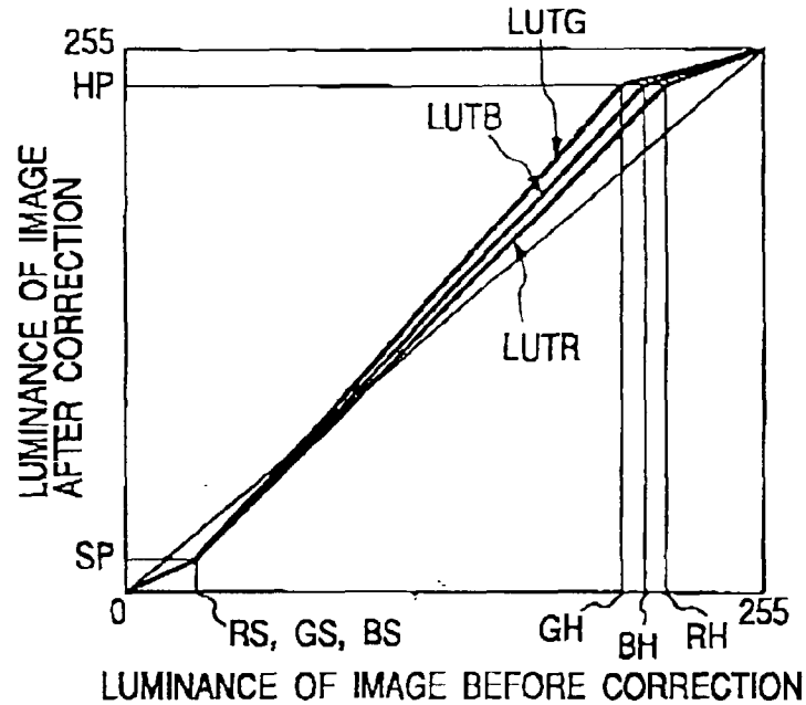
FIG. 17A LUT FOR CORRECTING COLOR FOG AND CONTRAST
