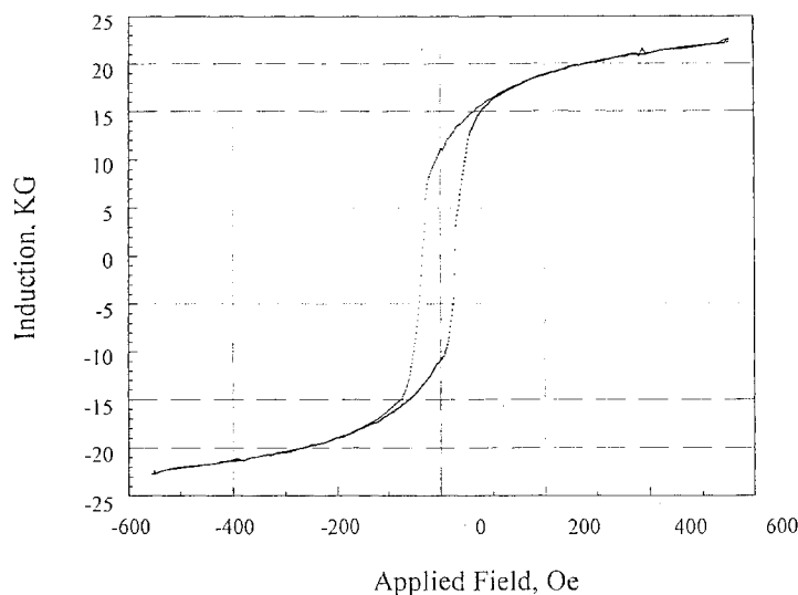
Figure 7: Alloy Example 1 Solution at 1610 ± 10 °F Aged at 950 ± 10 °F for 24 Hrs.
