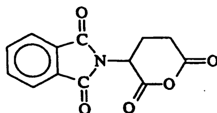
phthaloyl glutamic anhydride (PGA)
