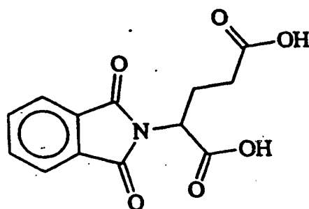
phthaloyl glutamic acid (PG Acid)
