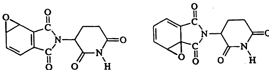
Epoxides of thalidomide
