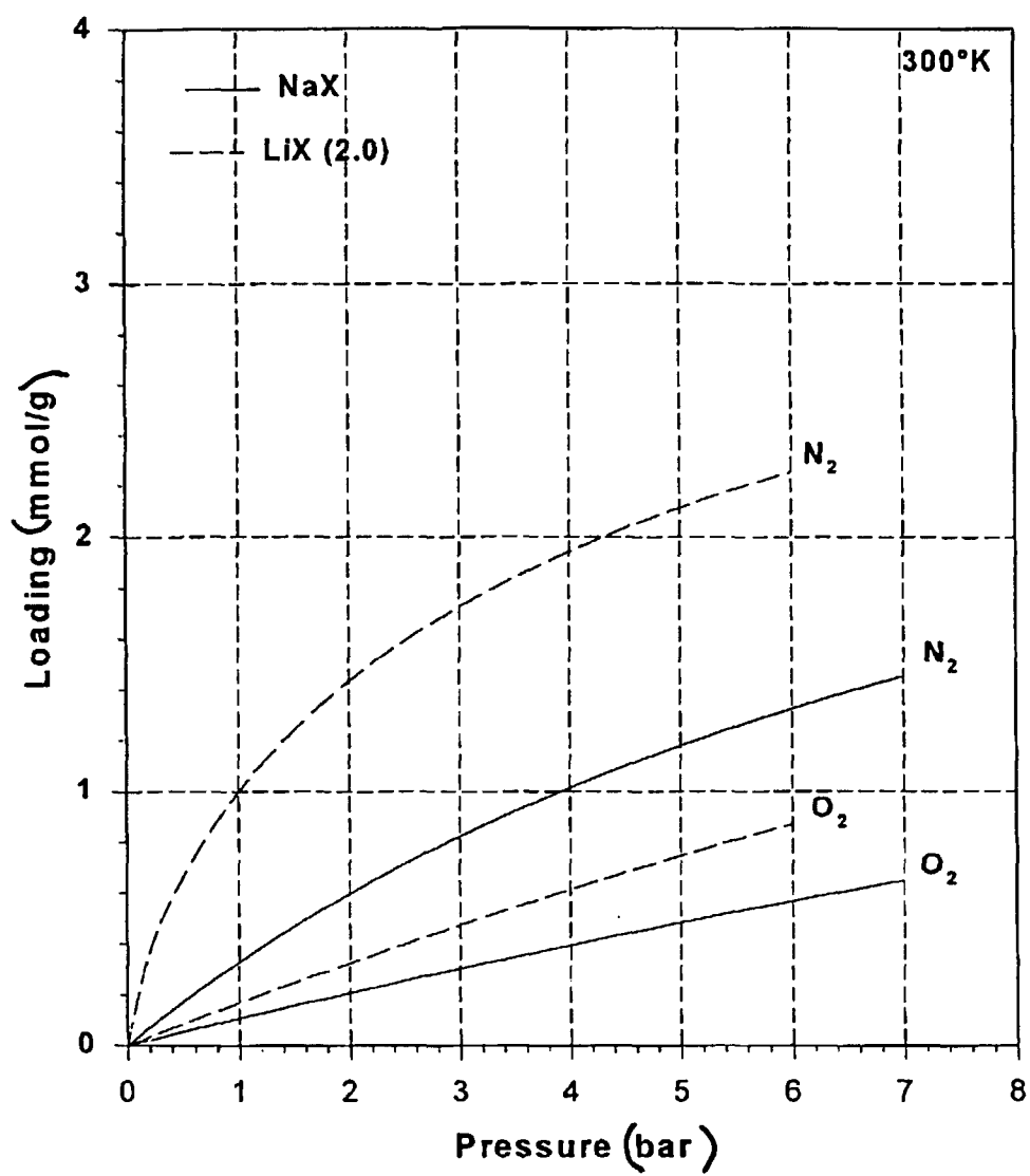
Figure 1 Adsorption Isotherms
