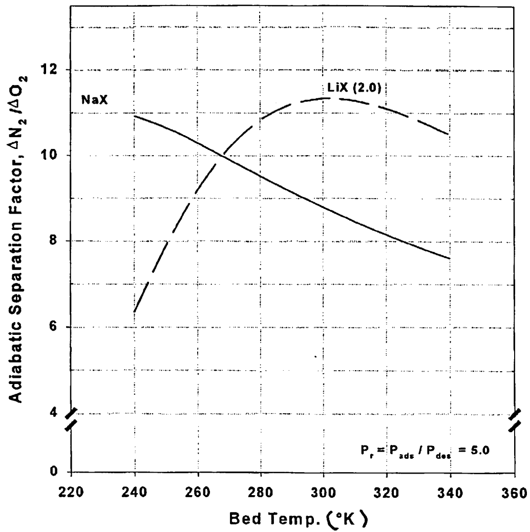
Figure 4 Variation of Adiabatic Separation Factor with Bed Temperature
