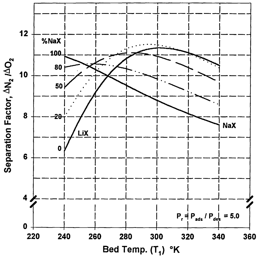
Figure 6 Variation of Separation Factor with Bed Temperature for LiX/NaX (2.0) Mixtures
