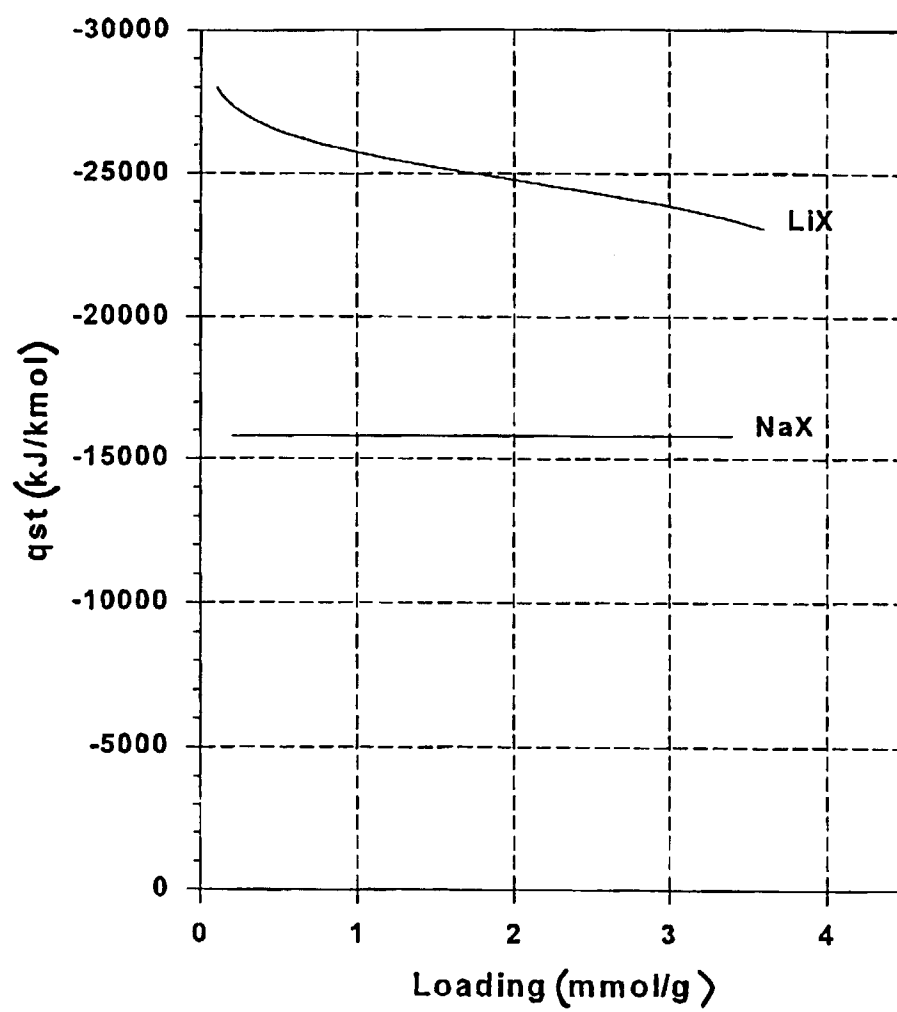
Figure 2 Isosteric Heat of Adsorption: N_2
