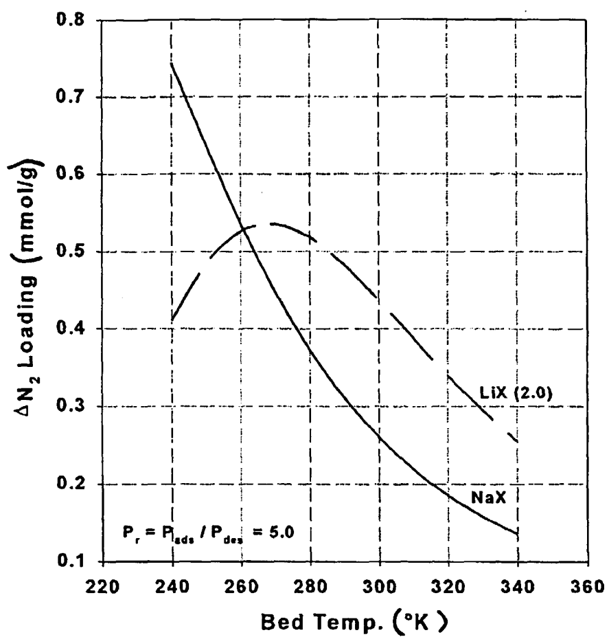
Figure 5 Variation of Adiabatic N 2 Working Capacity with Bed Temperature
