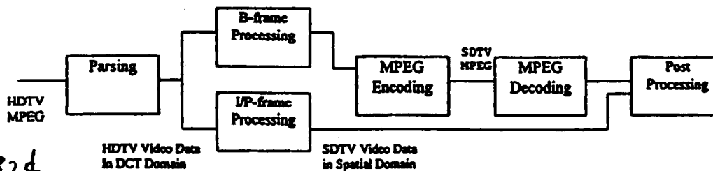
Transcoder Option 3: combination of options 1 and 2
