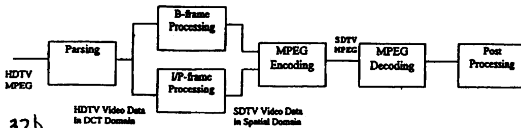
Transcoder Option 1: utilizing existing SDTV MPEG decoder
