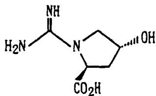
Compound (2): N-Amidino-L-proline
