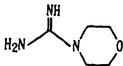
Compound (5): 4-Morpholinecarboxamidine
