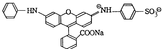
C.I. Acid Violet 30
