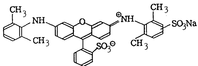
C.I. Acid Red 289
