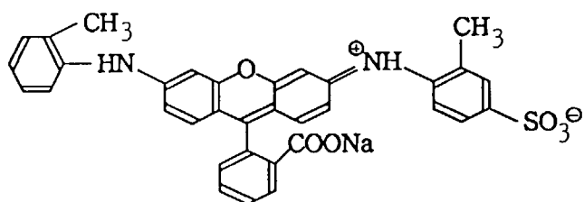
C.I. Acid Violet 9
