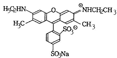
C.I. Acid Red 51
