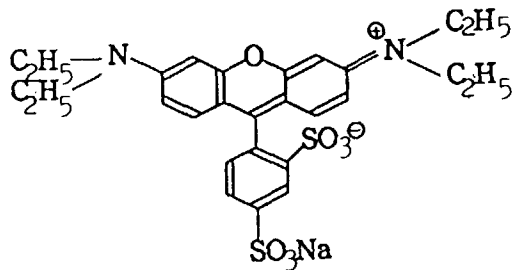
C.I. Acid Red 52
