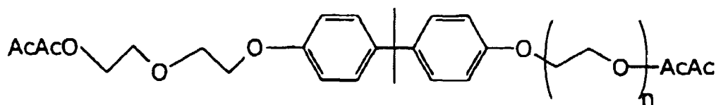
A + isomers
