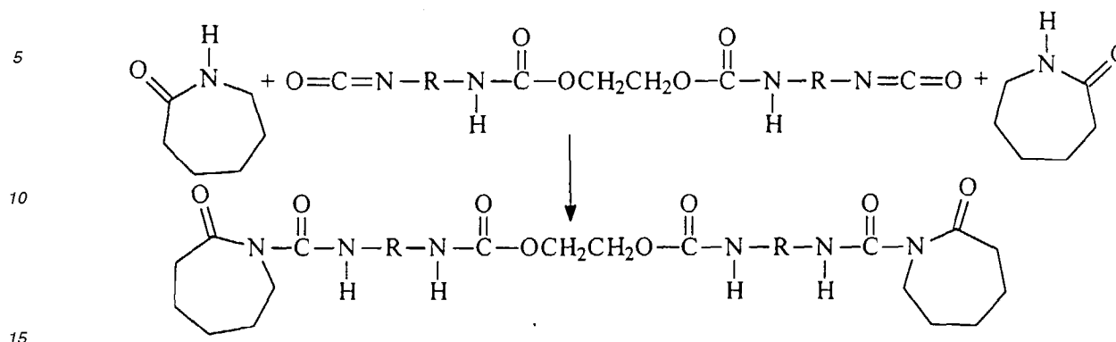
Scheme 3: Formation of \epsilon -Caprolactam Blocked Isocyanate
