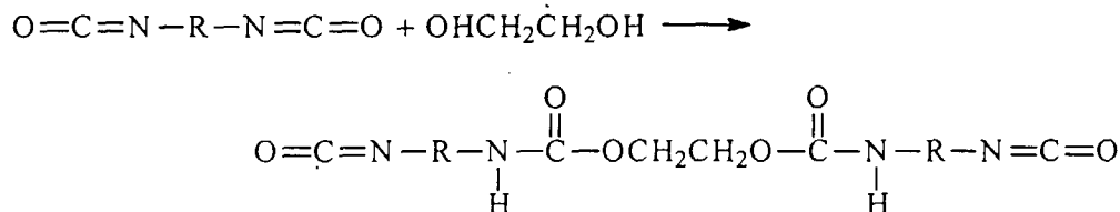
Scheme 2: Reaction of a diisocyanate with a diol to form an isocyanate terminated adduct
