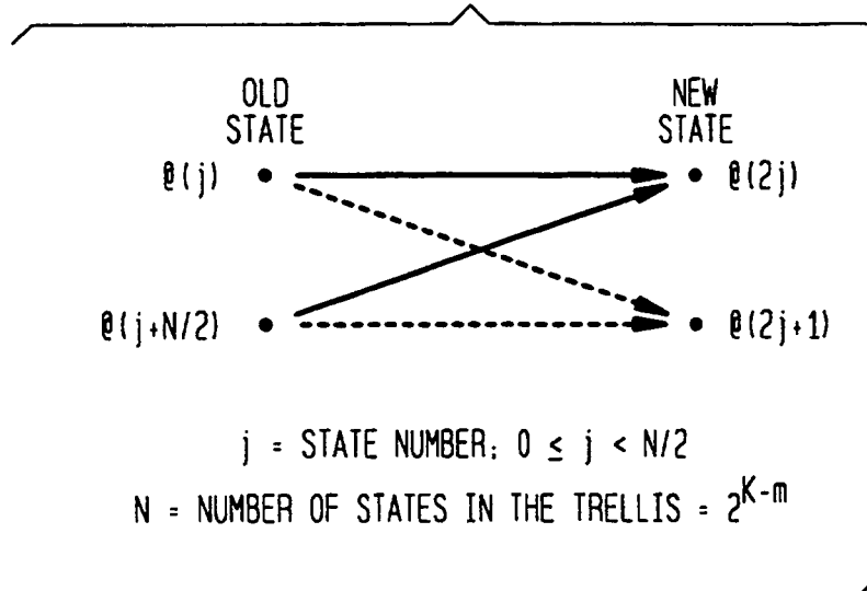
FIG. 2 (PRIOR ART)
