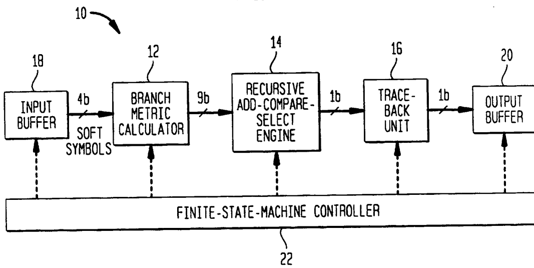
FIG. 5 (PRIOR ART)
