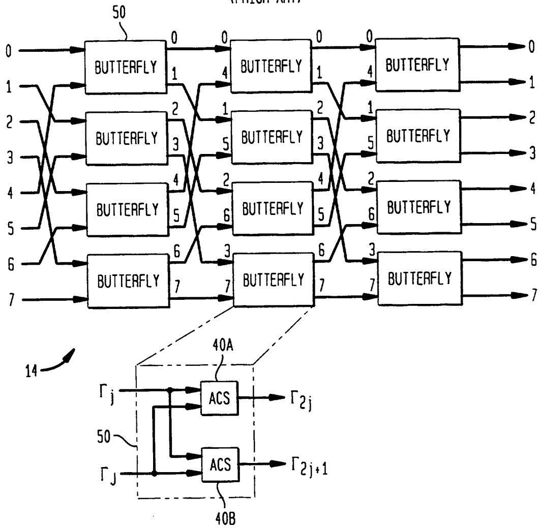
FIG. 7C (PRIOR ART)
