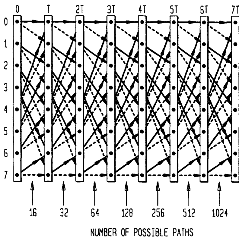
FIG. 4 (PRIOR ART)
