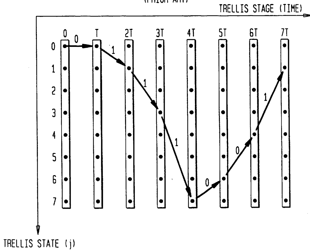
FIG. 3 (PRIOR ART)
