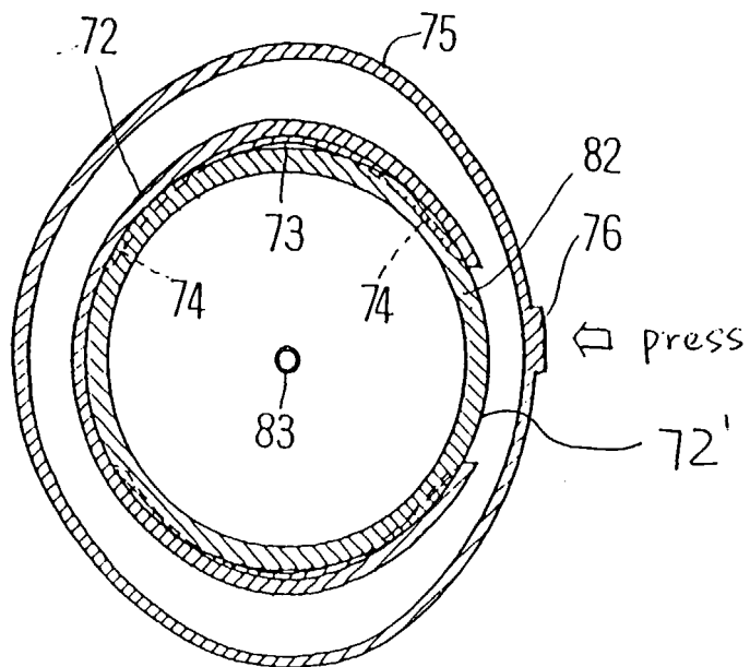
FIG. 6C PRIOR ART
