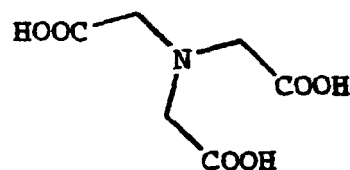
Glycine-N,N-diacetic acid
