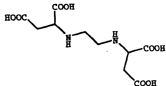
Ethylenediaminedisuccinic acid
