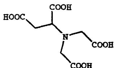
Glycine-N,N-diacetic acid
