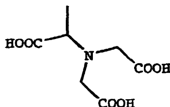
\beta -Alanine-N,N-diacetic acid
