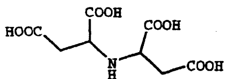
Iminodisuccinic acid
