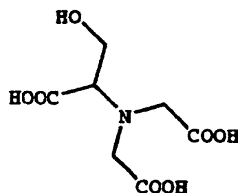
Serine-N,N-diacetic acid
