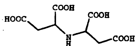
Iminodisuccinic acid
