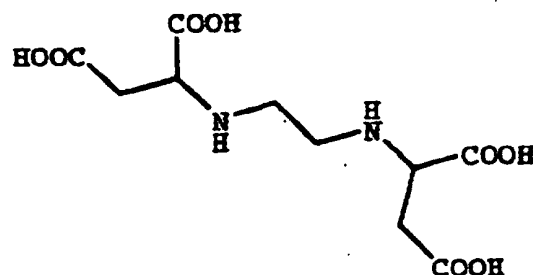
Ethylenediaminedisuccinic acid
