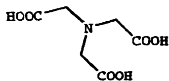
Glycine-N,N-diacetic acid
