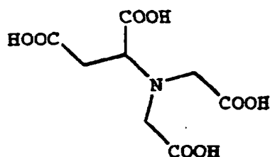
Glycine-N,N-diacetic acid
