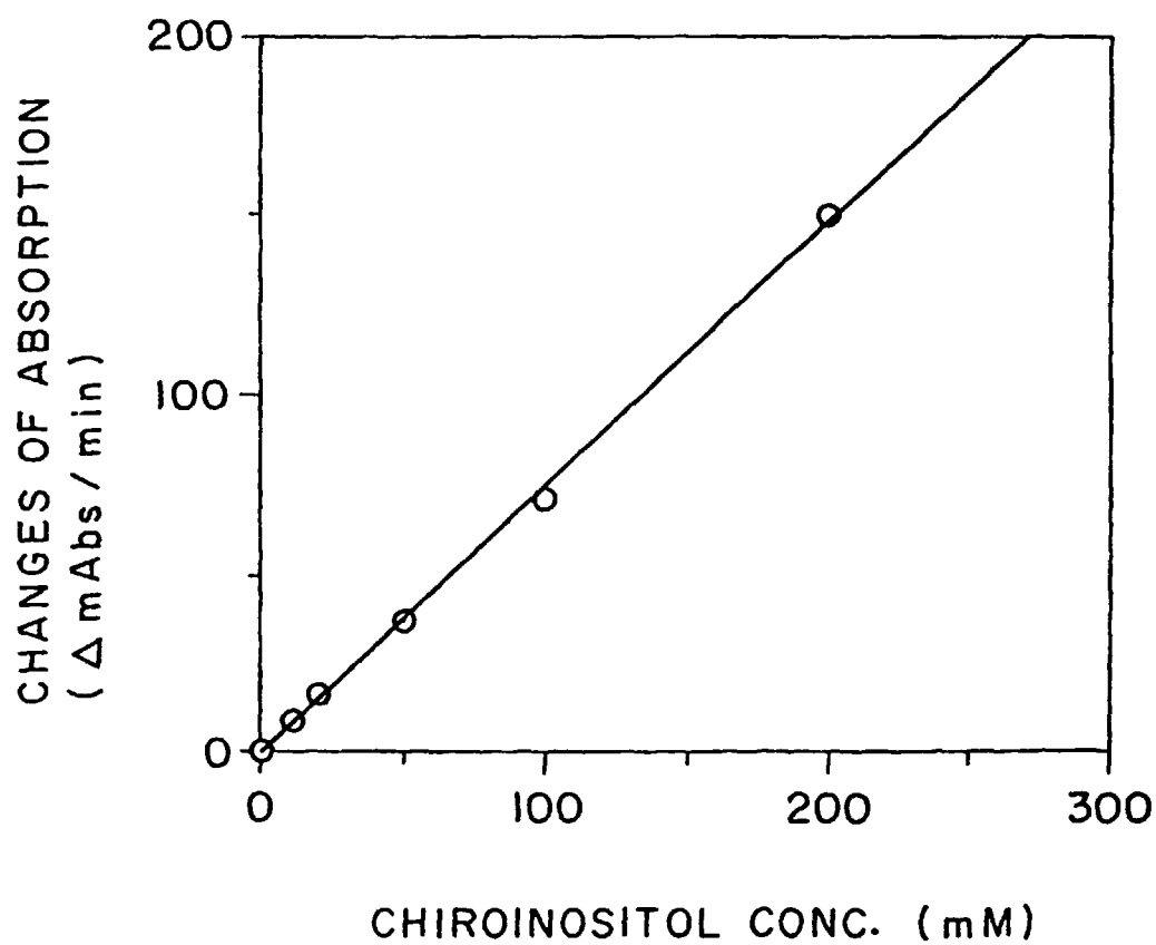
CALIBRATION CURVE (THIO-NADP / NADH)
