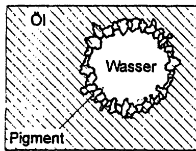
W/O-Pickering-Emulsion
