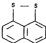
(1,8 naphthalene disulfide)
