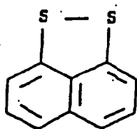
(1,8 naphthalene disulfide)
