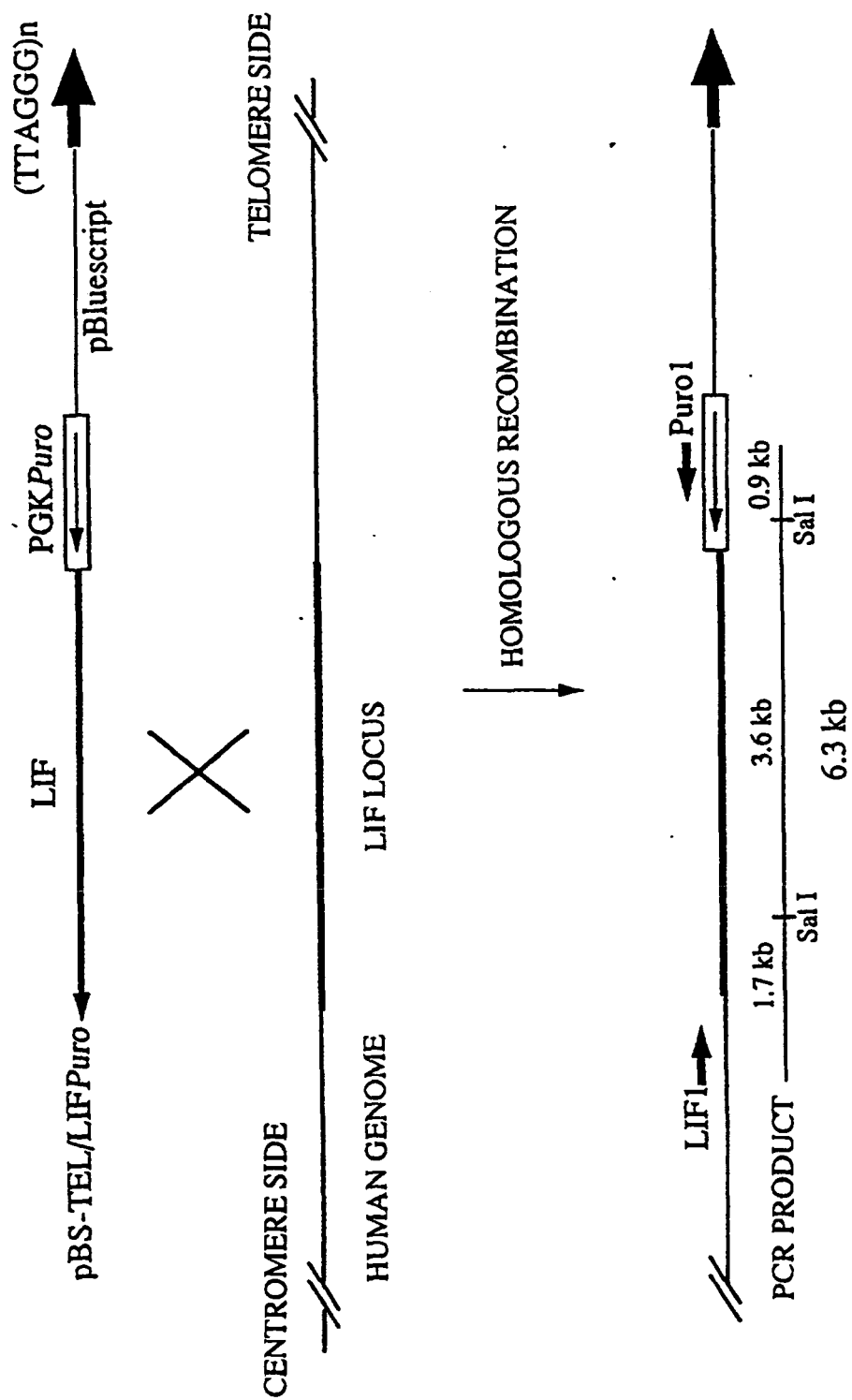
FIG. 47 IDENTIFICATION OF HOMOLOGOUS RECOMBINANT IN LIF LOCUS
