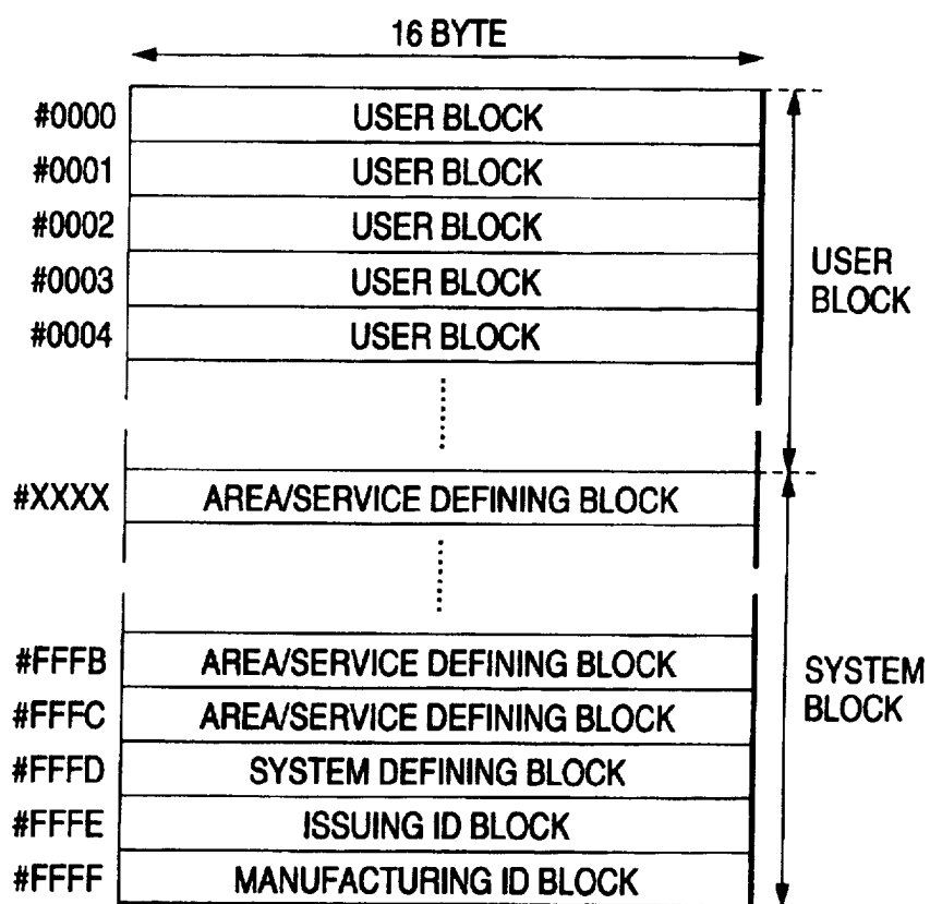
LOGICAL FORMAT OF EEPROM 66
