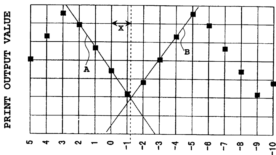
RELATIONSHIP BETWEEN RELATIVE POSITION SHIFTING AMOUNT IN FORWARD/REVERSE SCANS [PIXEL]
