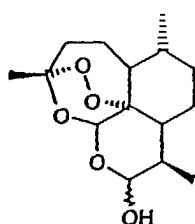
Dihydroartemisinin 2
