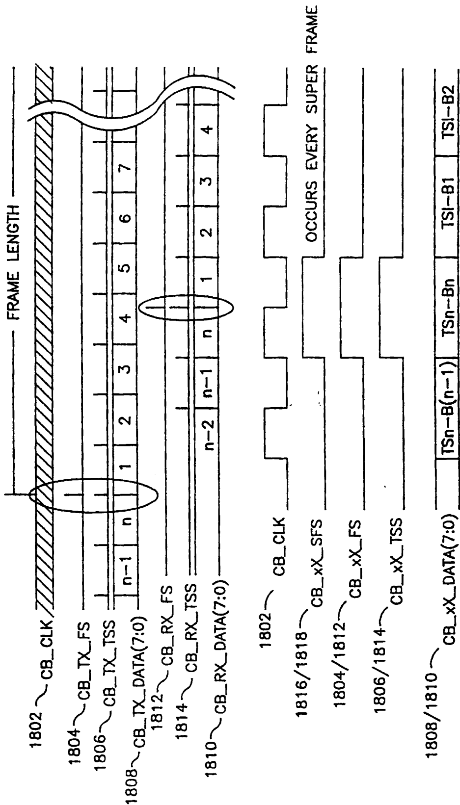
Fig. 18 CELL BUS TIMING
