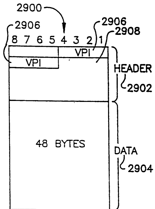
TDM CELL
