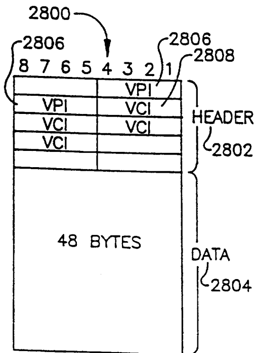
ATM CELL
