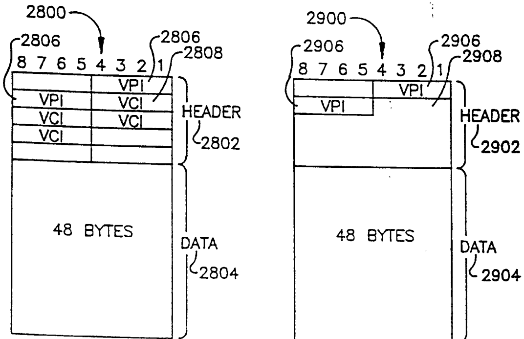
ATM CELL
